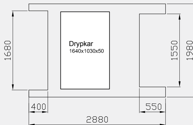
Beton fundament t=200 mm
