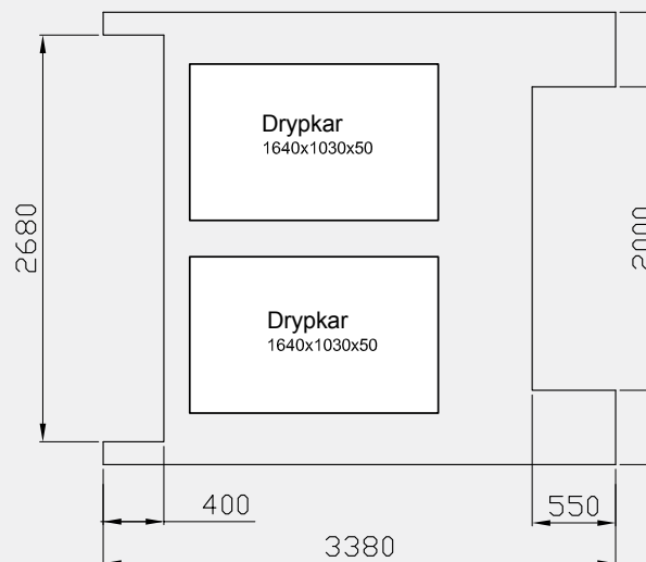
Beton fundament t=200 mm
