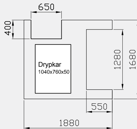
Beton fundament t=200 mm
